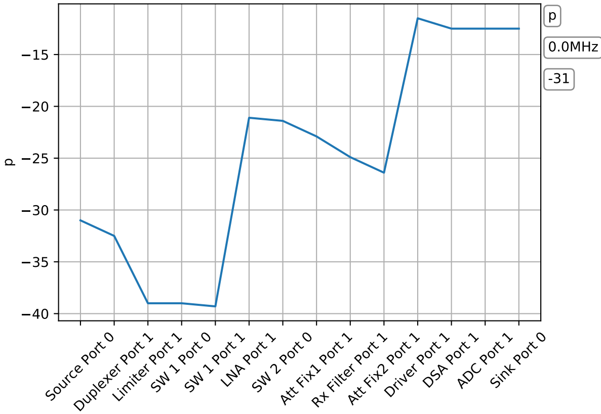
Performance: freq=0.0MHz, Pin=-31.0dBm
